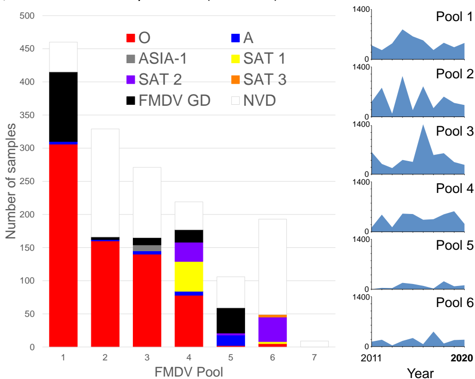
Figure 4: Representation of different FMDV serotypes detected in samples tested from the FMD endemic pools by the OIE/FAO FMD Laboratory Network during 2020 (NB: Figure 1 shows the geographical coverage of each pool; NVD = no virus detected; GD = genome detected by RT-PCR). Right-hand panels display historical trends for each of the pools (since 2011). NB; submission from Pool 7 are low and these data are not shown.
