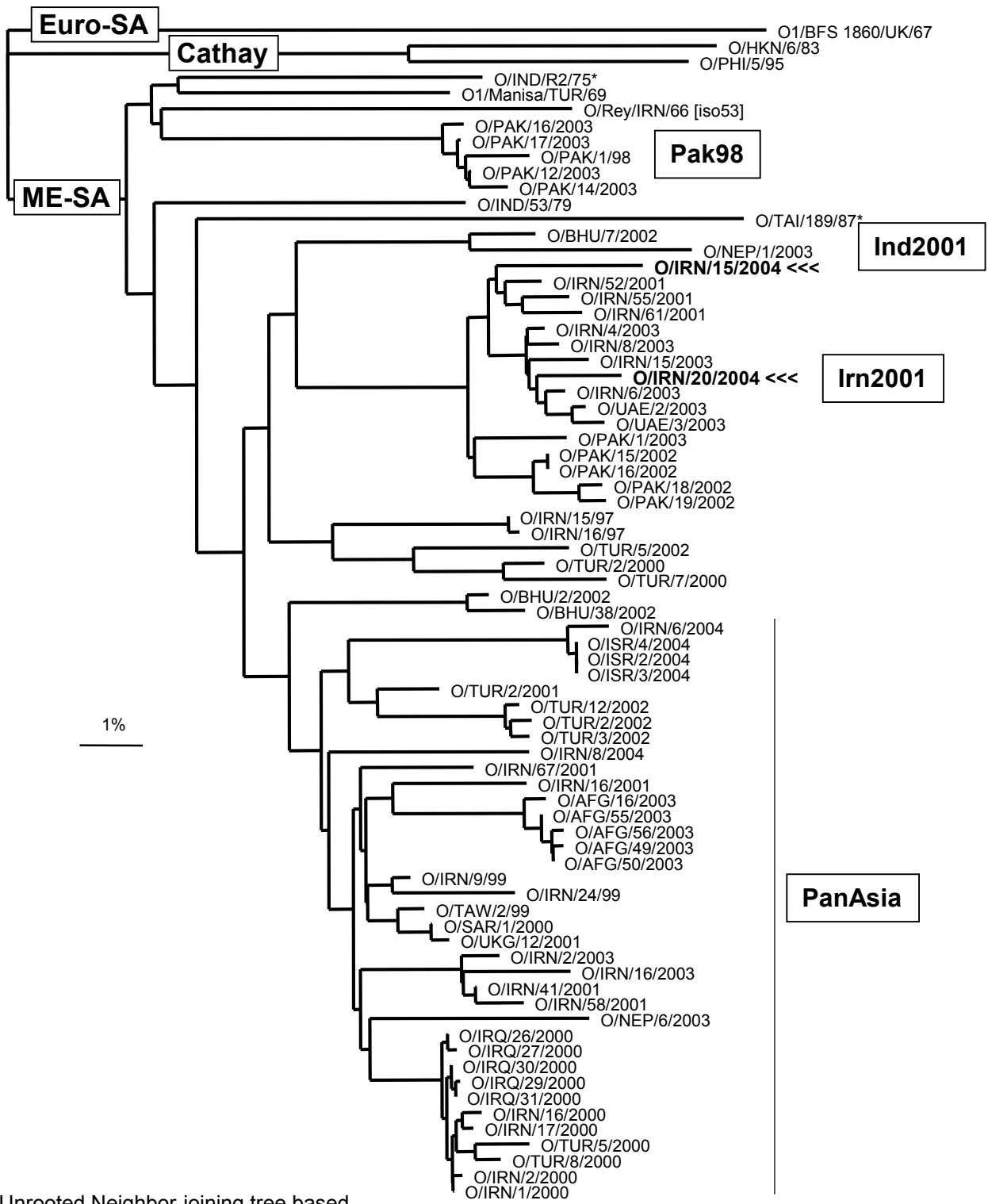
Unrooted Neighbor-joining tree based on a comparison of the complete VP1 gene. The tree was outgroup-rooted using O1/BFS 1860/UK/67.
